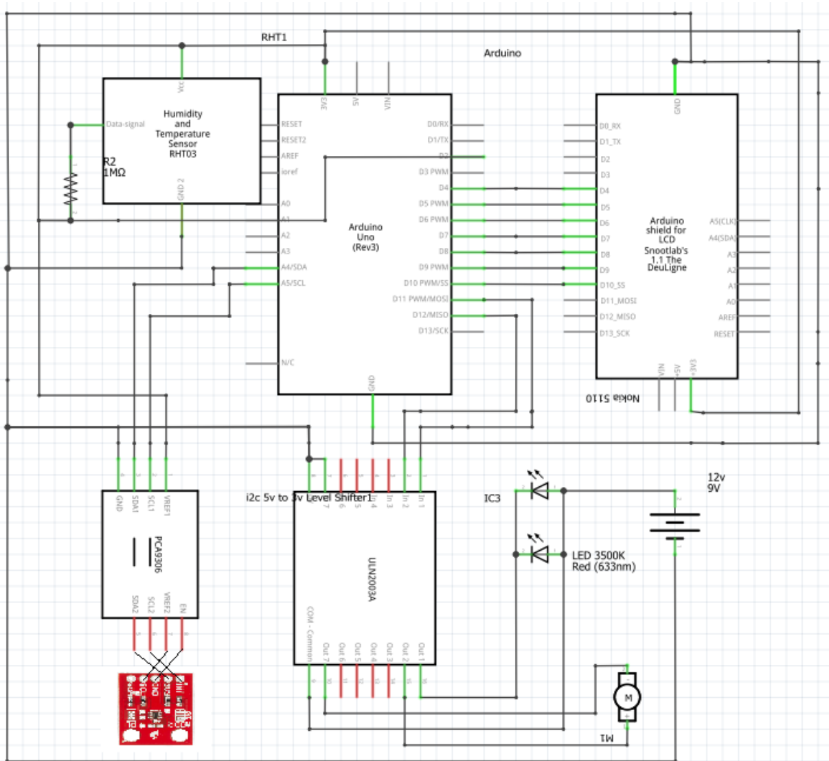
Figure 52 - Electronic schematic 1 (42)
