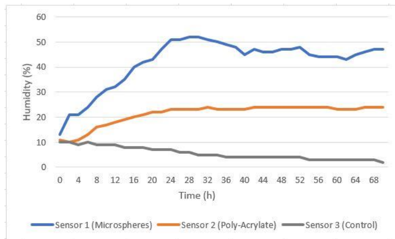
Figure 60 - Results of the soil test (47)
