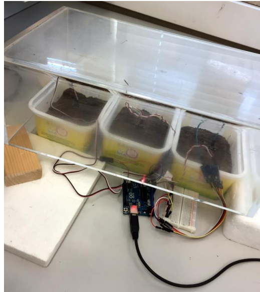
Figure 59 - Setup of the soil tests (46)
