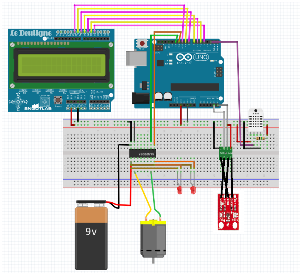
Figure 53 - Electronic schematic 2 (43)
