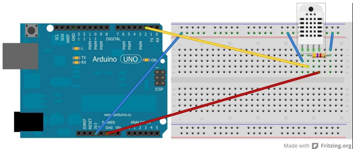
Figure 54 - Humidity and temperature sensor test schematic (44)
