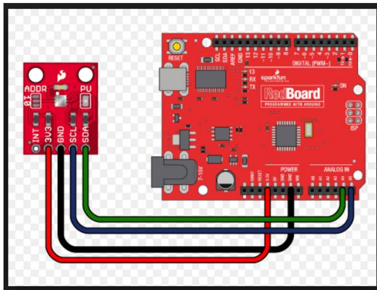
Figure 57 - Schematic system TSL2165 (45)
